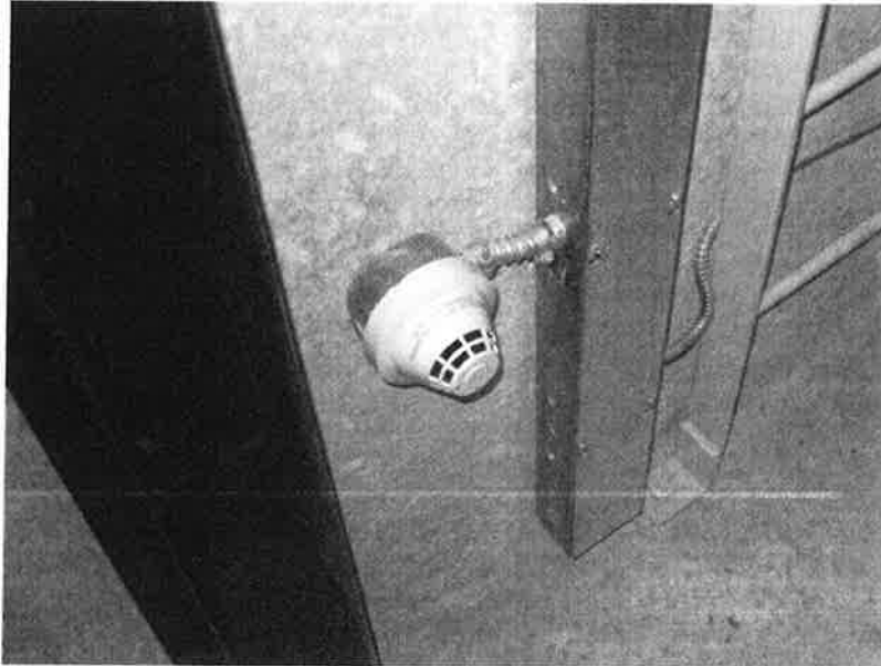
Heat Sensor in Elevator Shaft Lowest Machinery or Equipment Servicing Building
